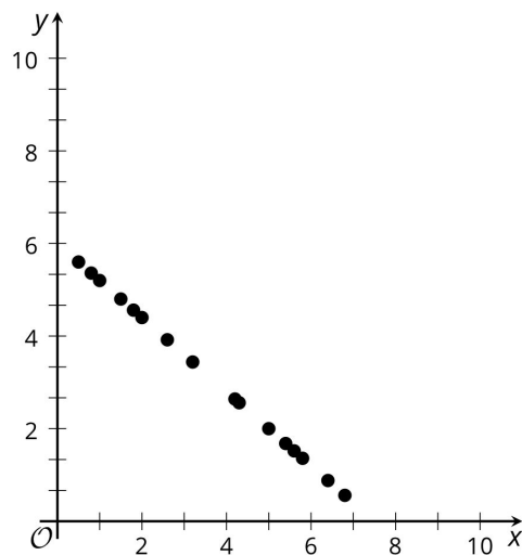
Card Sort: Scatter Plot Fit D
